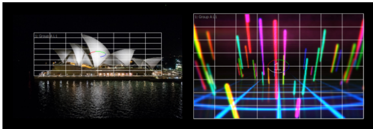
mapping_tracer_assistant.beyondlayout
